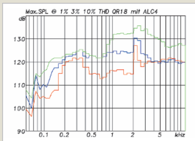
Pict.6: Maximum SPL of the QR18 referred to 1m distance at 1% (red), 3% (blue) and 10% (green) THD. The maximum power was 1,720W into 40hm.
