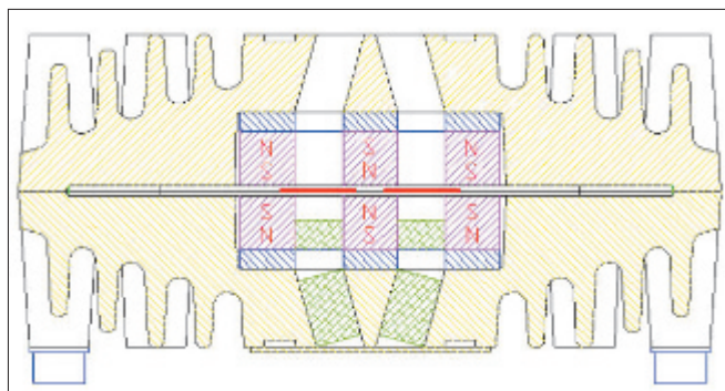
Cross-section drawing of the RBN-tweeter with aluminium casing (yellow), Neodymium magnets (red) and membrane (red) as well as the acoustic sink (green) on the back of the membrane.
