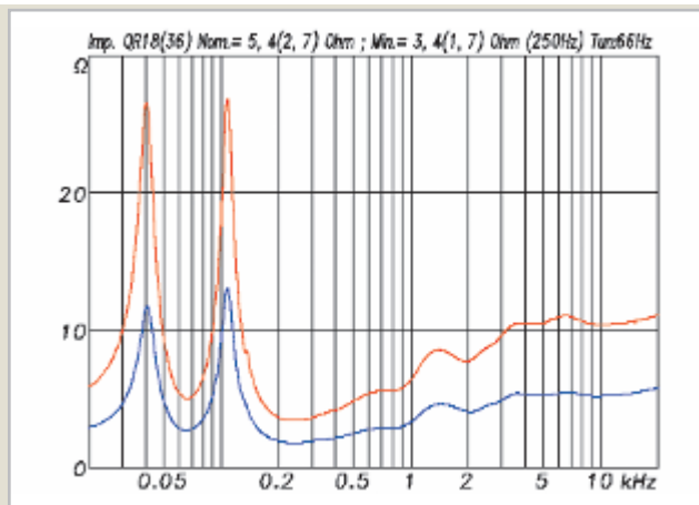
Pict.4: Impedance curve of QR18 (red) and QR36 (blue). The tuning frequency of the bass-reflex system is at around 66Hz in both cases. The impedance minima are rather low with 3.4 ohms and 1.7 ohms, so the QR18 should correctly be called a 4 ohms system and the QR36 a 2 ohms system. In the higher frequency range only the 12 ohms or 6 ohms respectively of the ribbon-tweeters matter.
