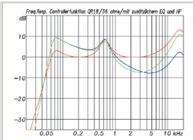
Pict.2: Controller and EQ functions for the Q-series. The red graph is equivalent to the filters on the controller card for the Alcons ALC amps. For the listening tests some additional filters were set, which finally resulted in the blue graph for the QR18 and the green graph for the QR36. The additional filters were a high- and low-shelving filter each as well as a highpass filter with a Q-factor of 2.0 at 64 Hz. During the listening tests the Q-factor was reduced to 1.2 since the bass rise seemed to pronounced.
