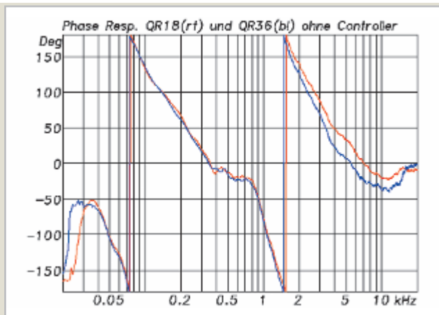
Pict.3: Phase response for QR18 (red) and QR36 (blue). The curves are almost identical except for the HF-range as was expected. The phase response is defined by a 360° shift at the low end of the frequency range caused by the acoustic highpass function of the 4th order of the bass-reflex enclosure and another 360° turn in the area of the cross-over frequency between tweeter and LF unit with a crossover of the 4th order.
