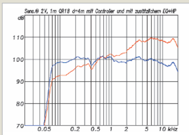
Pict.5: Frequency response of the QR18 with controller card in the amplifier (red) and with additional EQ following picture 2. Dedicated "flat" SDP controller-modules are available for any system configuration.
