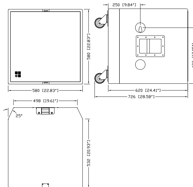
C7-TOP Abmessungen in mm [Zoll]
